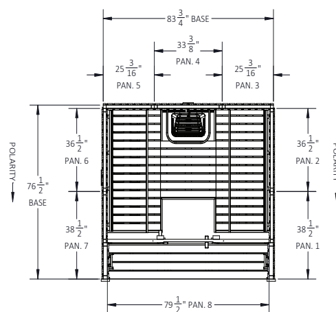
Top Down View w/ Interior Measurements
