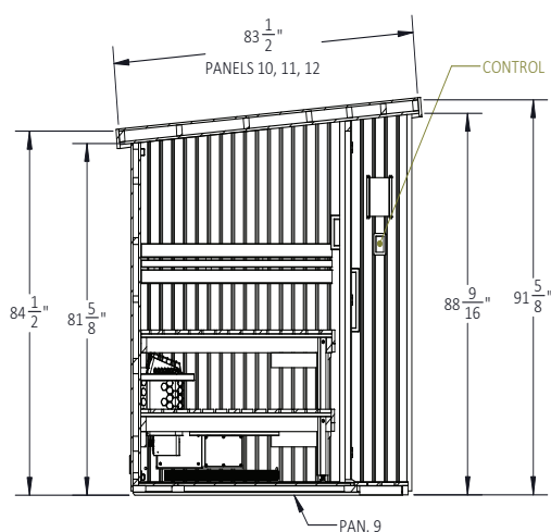
Interior Left Wall
