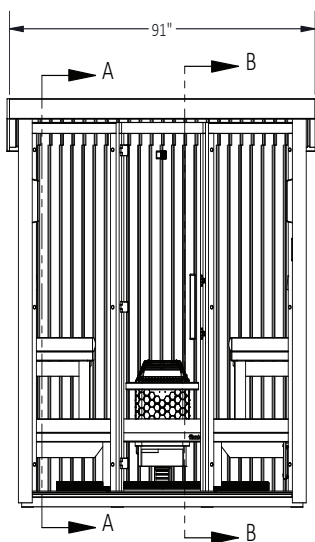
Exterior Front Wall
